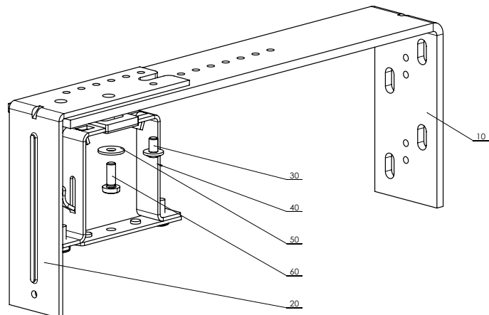
Adjustable double bracket – fixed 306 – 368 mm P 010/47 (2-01805-0000)
