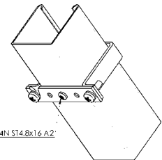
Sloped Exterior Blind 2-01077-XXXX-A
