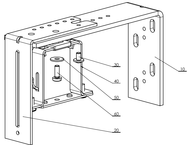
Adjustable double bracket – fixed 206 – 268 mm P 010/45 (2-01803-0000)
