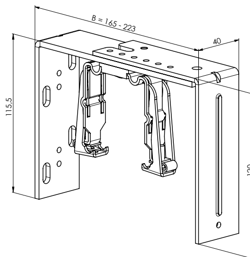
Blind bracket - long, adjustable and mechanical 165 - 223 mm P 009/22 (2-01391)
