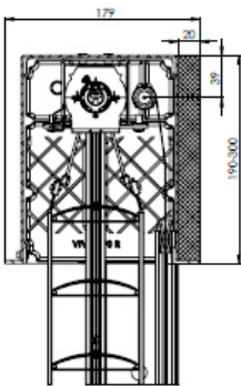
Section of built-in self-supporting blind Viva (prepared for polystyrene from the front + styrodur 20 from the back)
