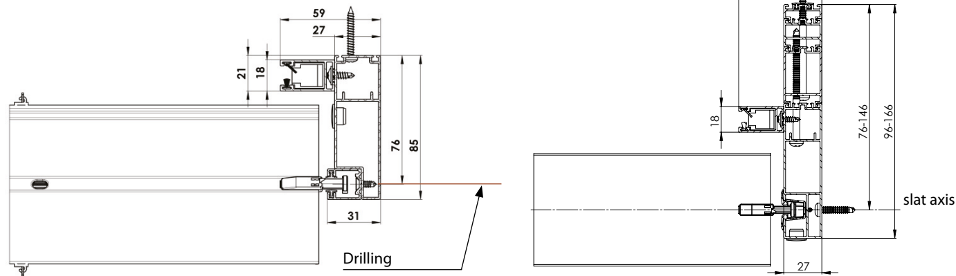
Cross of the detail for insect screens
